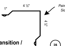
3 Transition / Endwall Trim
