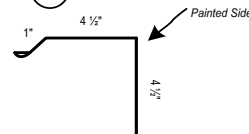
25 Mini-Gable Trim
