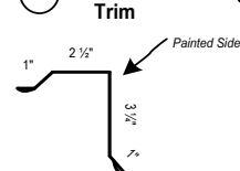
25 Mini-Gable Trim
