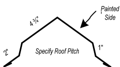
1 14" Sculptured Ridge Cap
